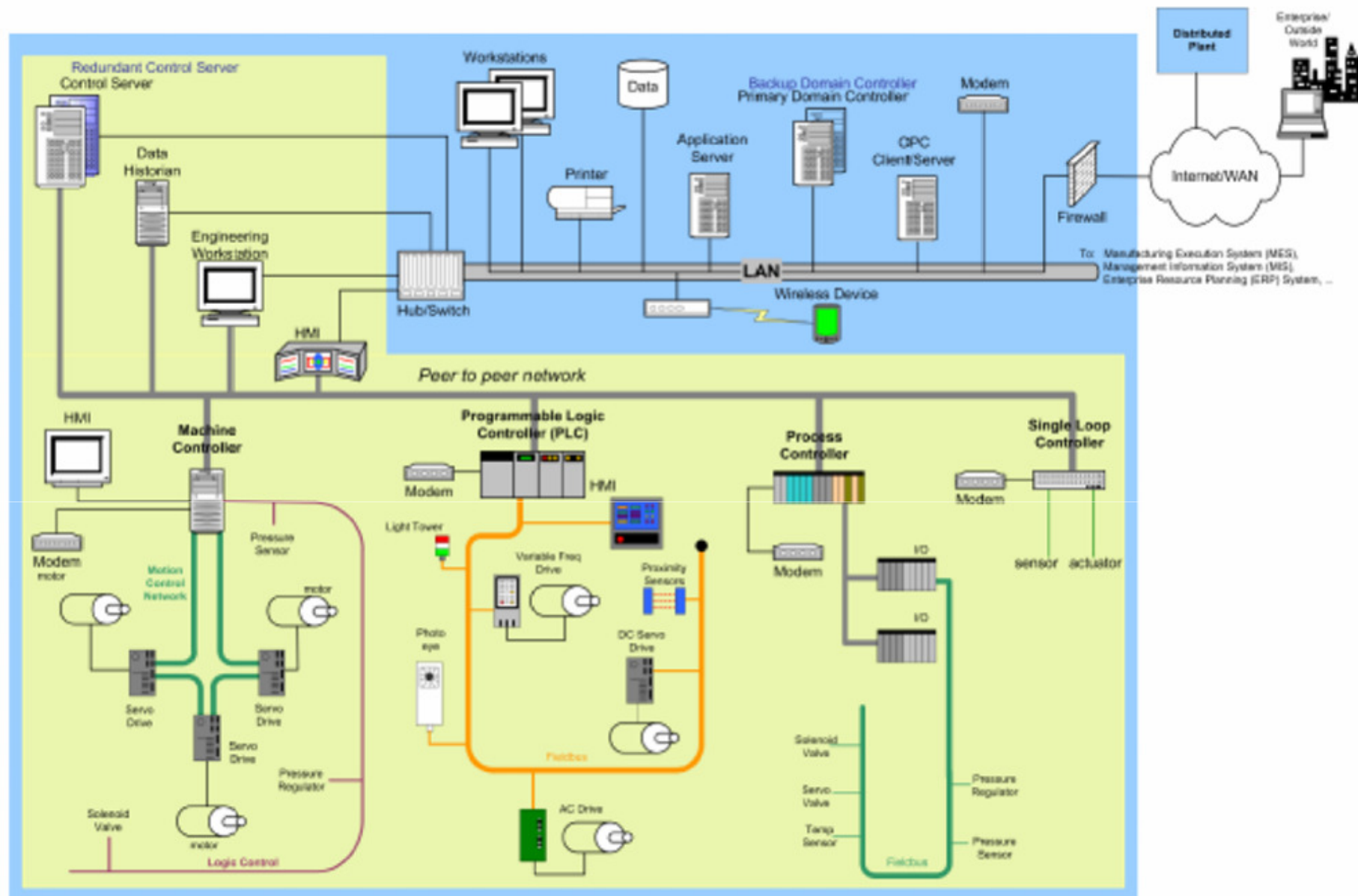
Figure 2: Generic Industrial Control System Network Architecture - DCS
