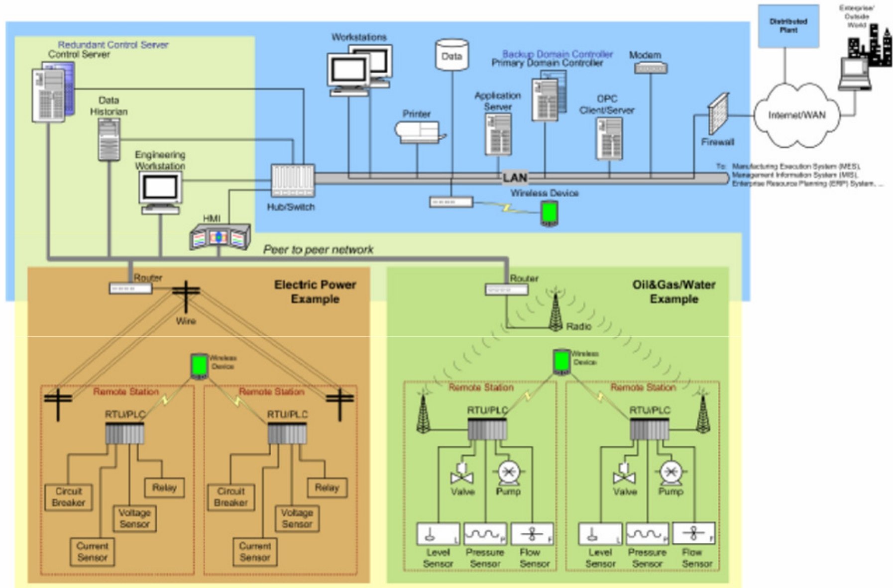
Figure 3: Generic Industrial Control System Network Architecture - SCADA
